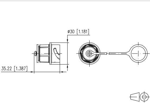
Dimensional drawing
