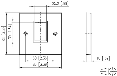
Dimensional drawing
