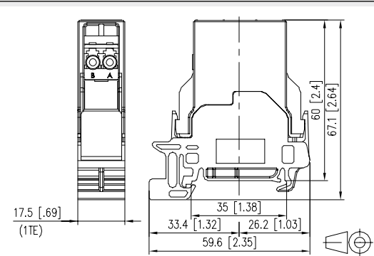
Dimensional drawing
