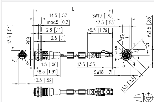
Dimensional drawing
