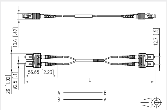
Dimensional drawing
