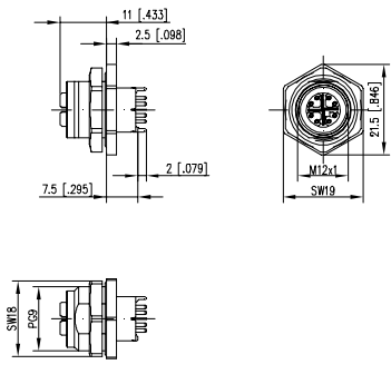
Dimensional drawing
