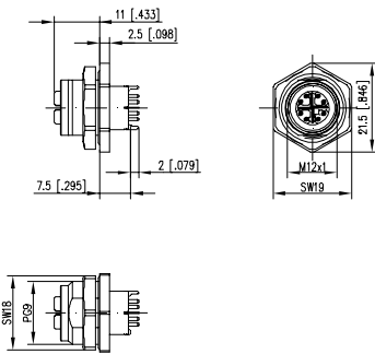
Dimensional drawing
