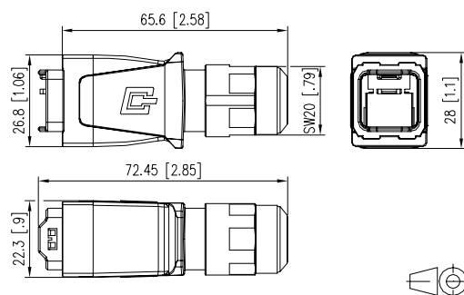
Dimensional drawing
