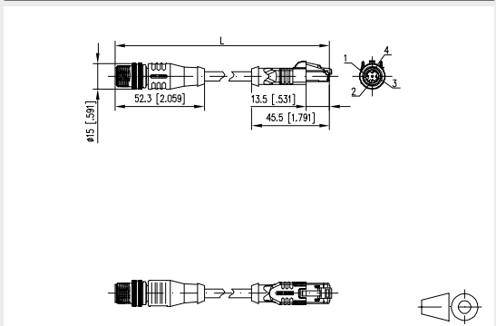
Dimensional drawing
