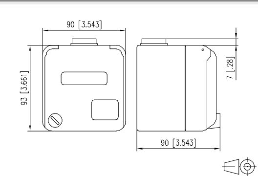
Dimensional drawing
