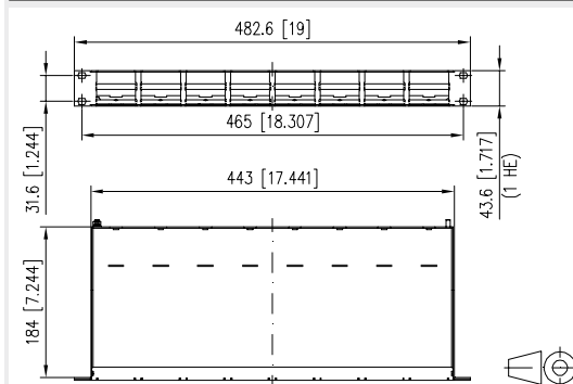
Dimensional drawing
