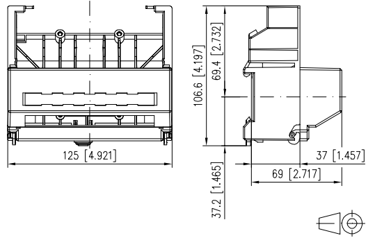
Dimensional drawing
