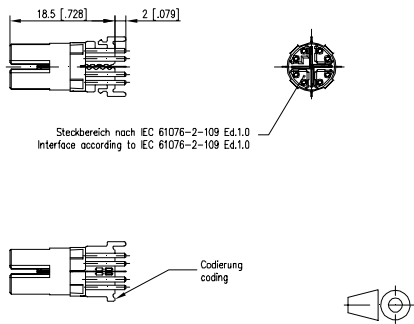
Dimensional drawing
